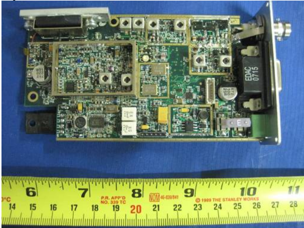
PCB Board-without RF shield Top View
