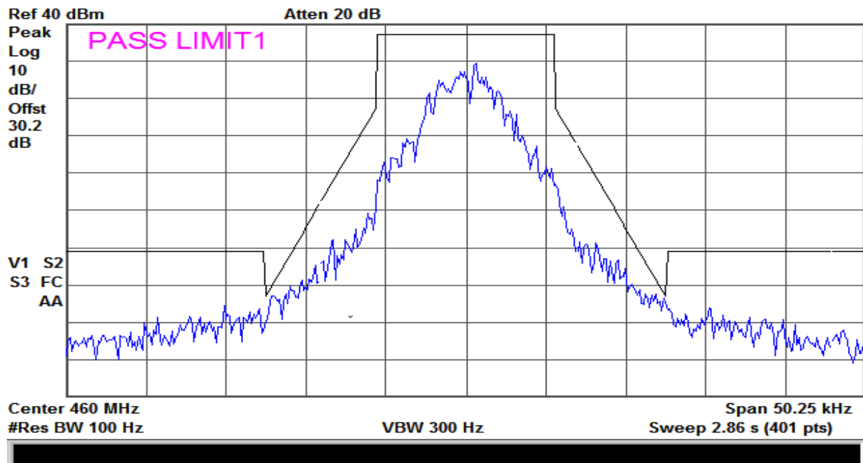
Plot 10 – Mid Chanel at Wideband Band 12.5 kHz Spacing – Mask D
