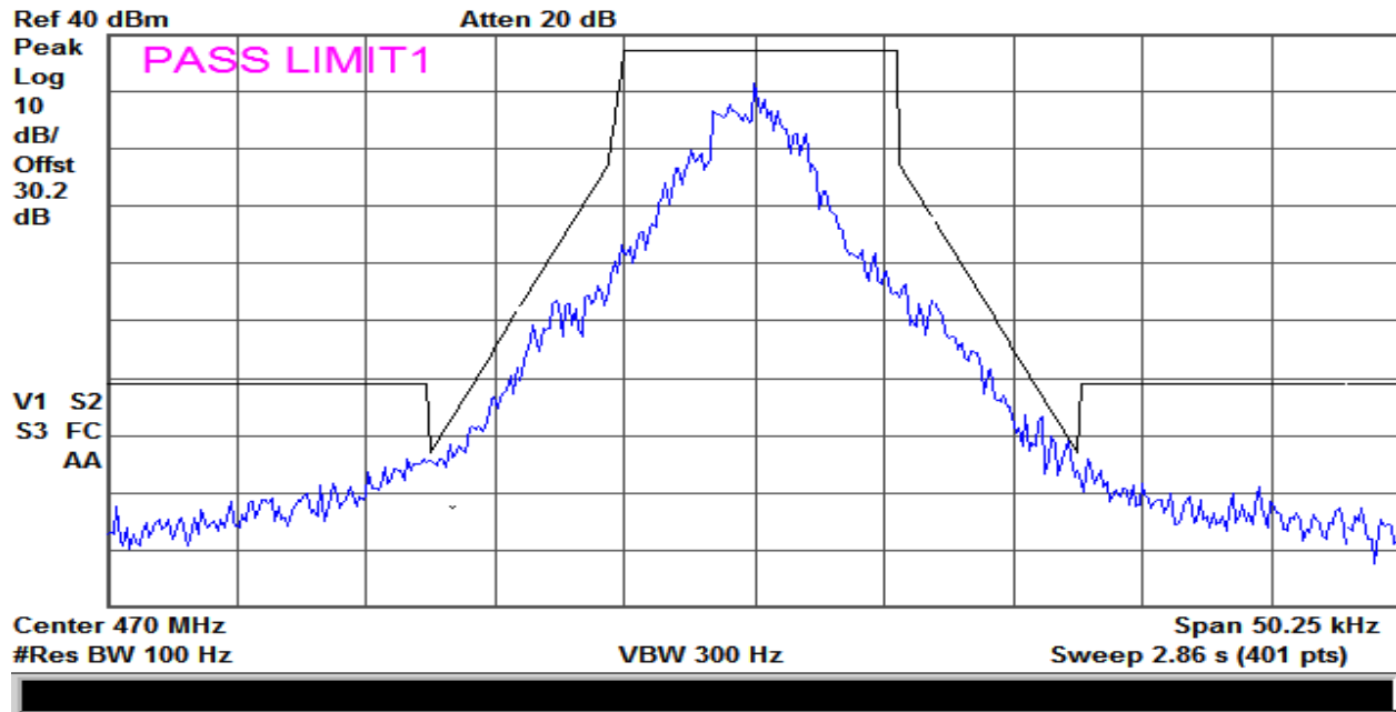
Plot 11 – High Chanel at Wideband Band 12.5 kHz Spacing – Mask D
