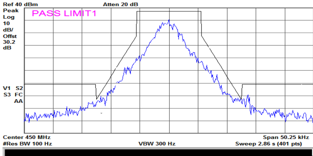
Plot 9 – Low Chanel at Wideband Band 12.5 kHz Spacing – Mask D
