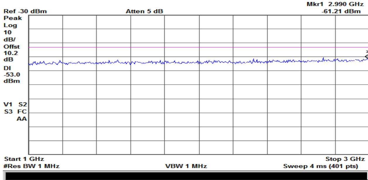
Plot 19 – Receiver Emission – For Industry Canada Only (RSS-GEN)
