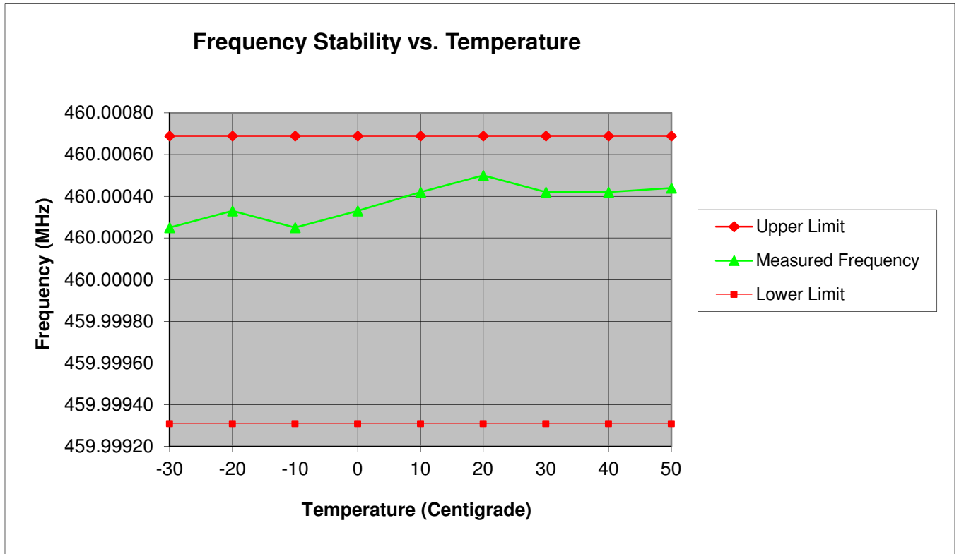
Plot 18 – Temperature vs Frequency
