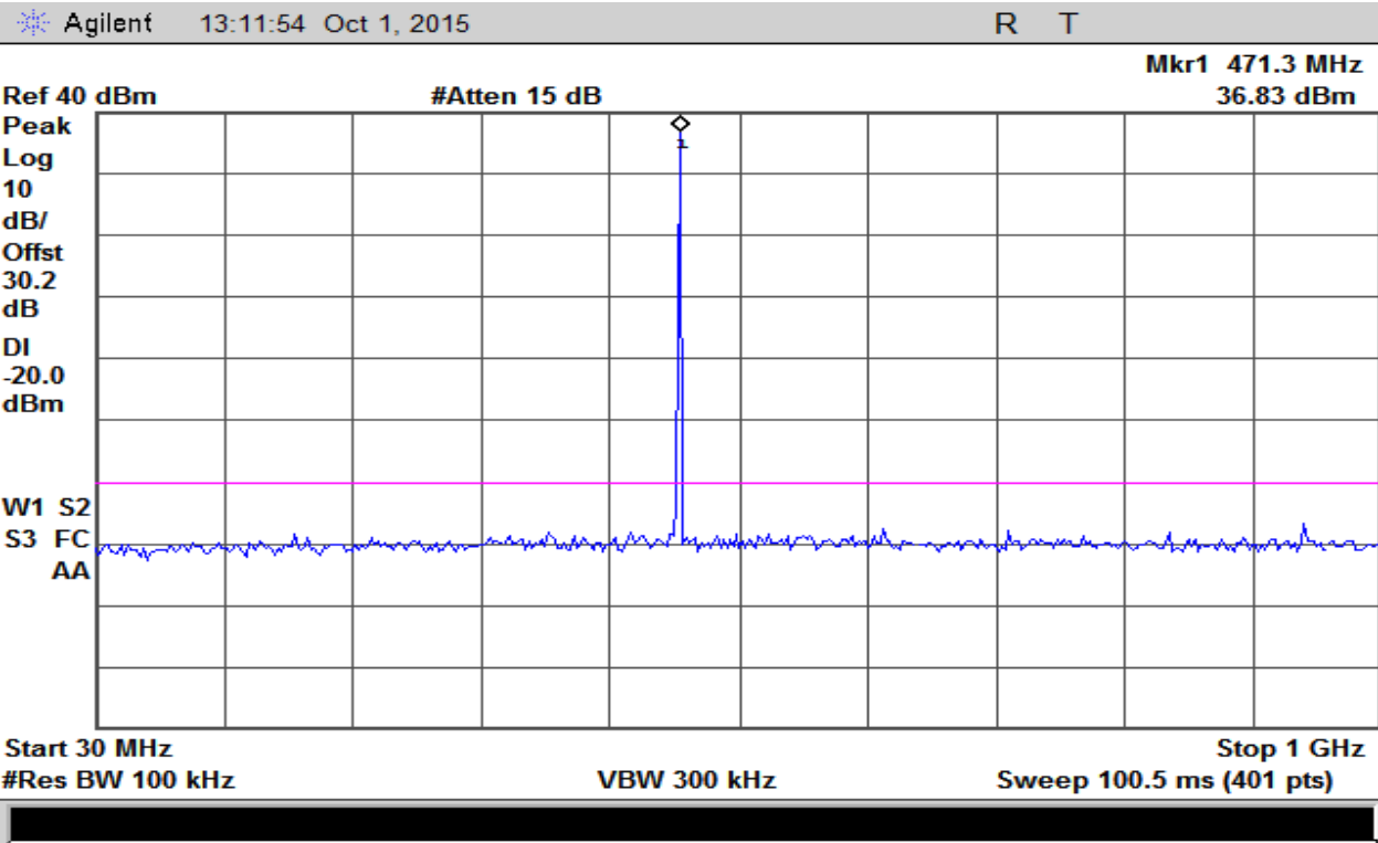
Plot 16 – High Band
