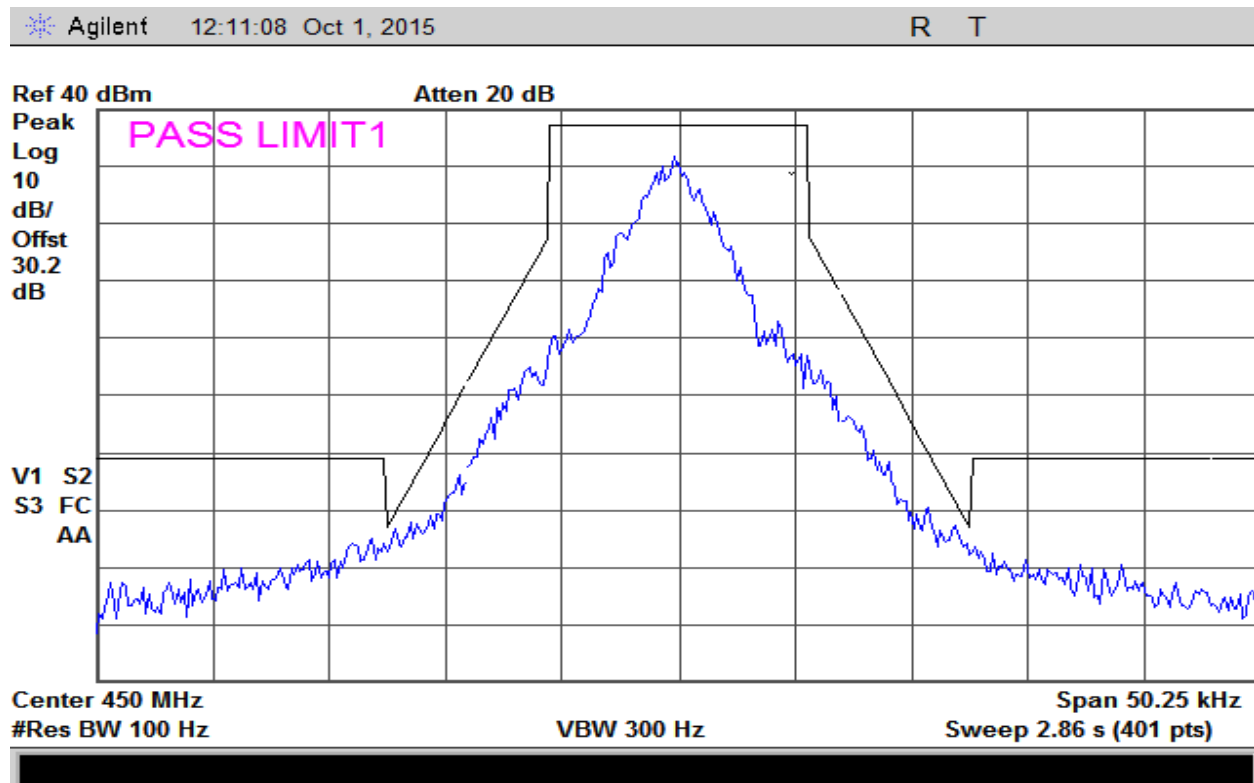
Plot 6 – Low Chanel at Narrow Band 12.5 kHz Spacing – Mask D
