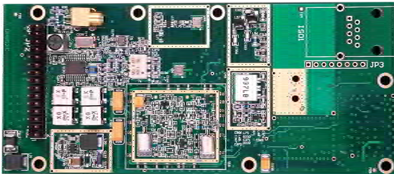
PCB RF Board – Bottom
