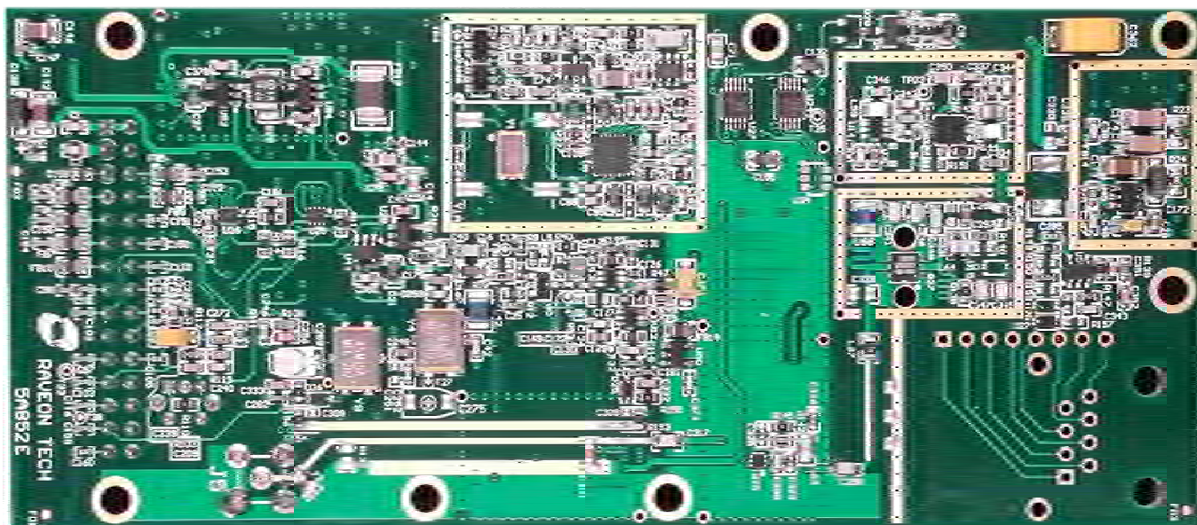
PCB RF Board - Top
