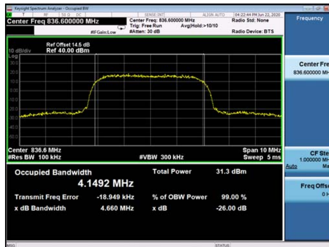
(Plot F2: WCDMA 850MHz Channel =4183 Occupied bandwidth)
