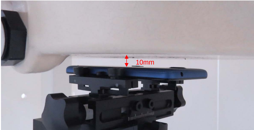
Picture 5: Back Side, the distance from handset to the bottom of the Phantom is 10mm
