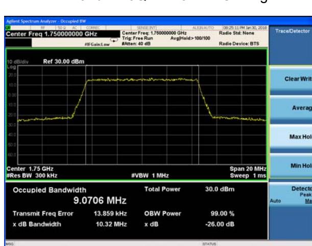
LTE Band 4 16QAM 10MHz CH-High
