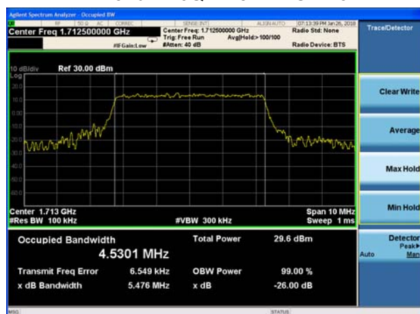
LTE Band 4 16QAM 5MHz CH-Low
