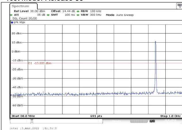
Channel 4132 30MHz~1GHz(dBm)
