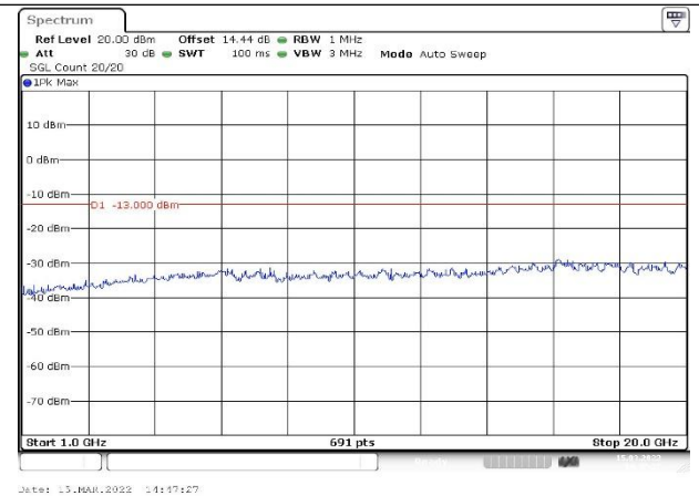
Channel 4132 1GHz~20GHz(dBm)
