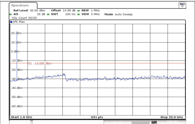
Channel 1312 1GHz~20GHz(dBm)
