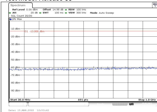
Channel 1312 30MHz~1GHz(dBm)
