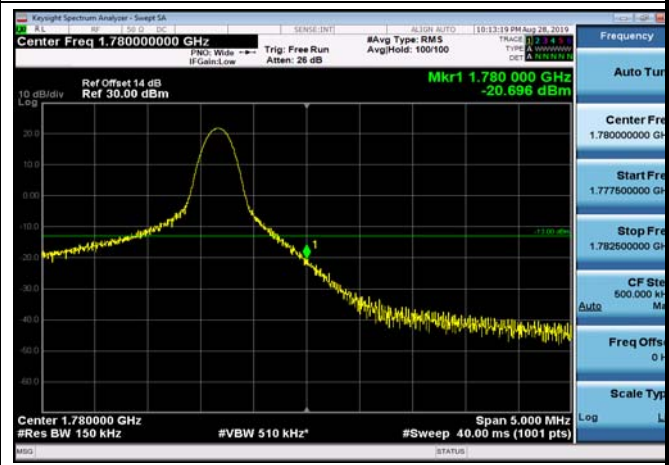
HighRange_FDD66_15MHz_1772.5_OneRB _high_Q16
