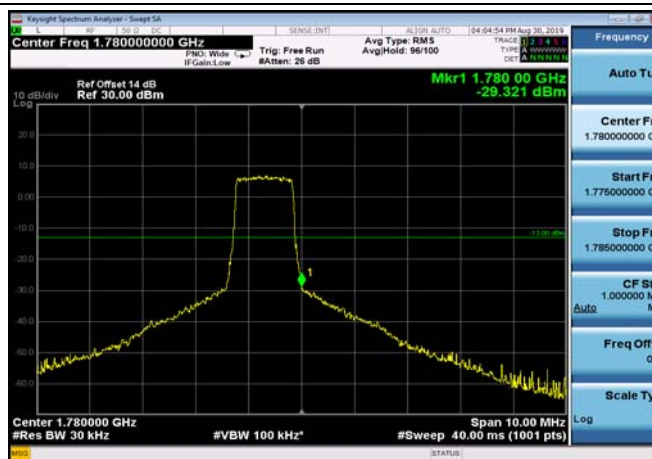
HighRange_FDD66_3MHz_1778.5_OneRB _high_Q16
