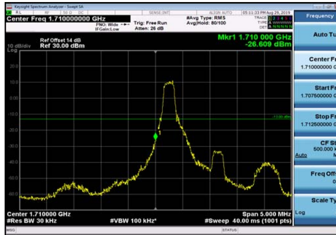
LowRange_FDD66_10MHz_1715_OneRB _low_QPSK
