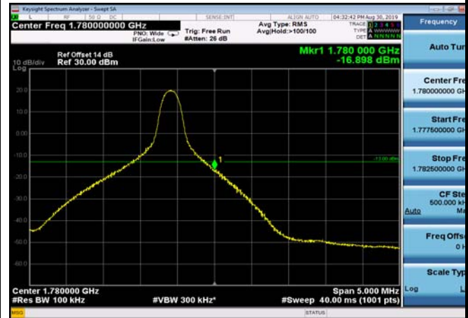
HighRange_FDD66_10MHz_1775_OneRB _high_Q16
