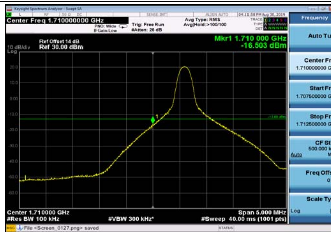
LowRange_FDD66_15MHz_1717.5_OneRB _low_QPSK
