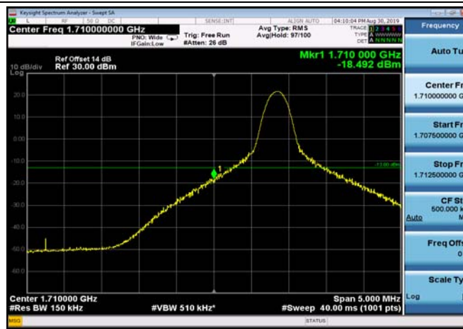
LowRange_FDD66_15MHz_1717.5_OneRB _low_QPSK
