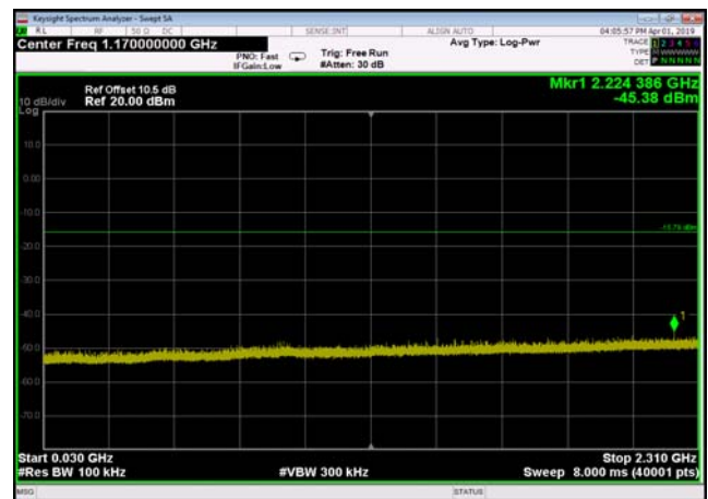
,Plot 3,30MHz~2310MHz-802.11g,2462MHz
