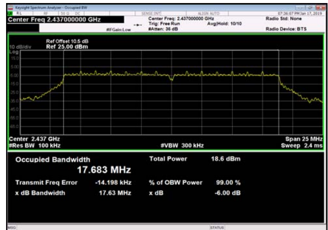
6dB Bandwidth-802.11n(HT20),2437MHz
