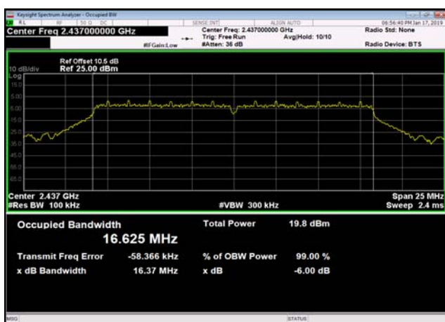
6dB Bandwidth-802.11g,2437MHz
