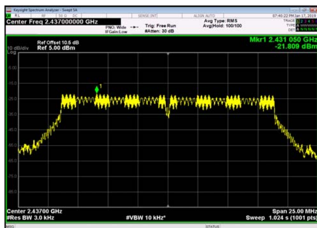
Power spectral density-802.11n(HT20) ,2437MHz
