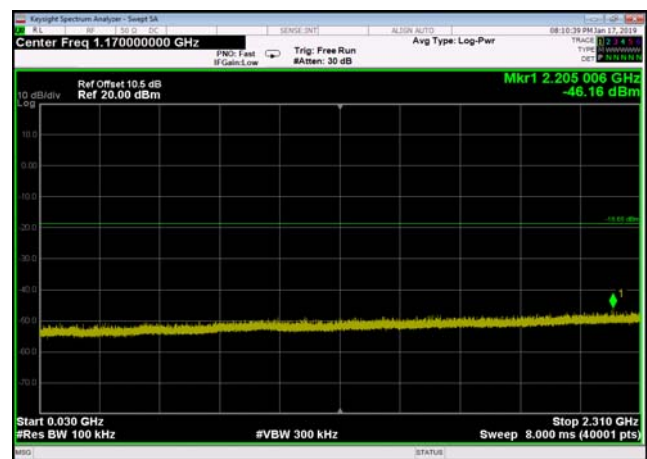
,Plot 3,30MHz~2310MHz-802.11g,2462MHz
