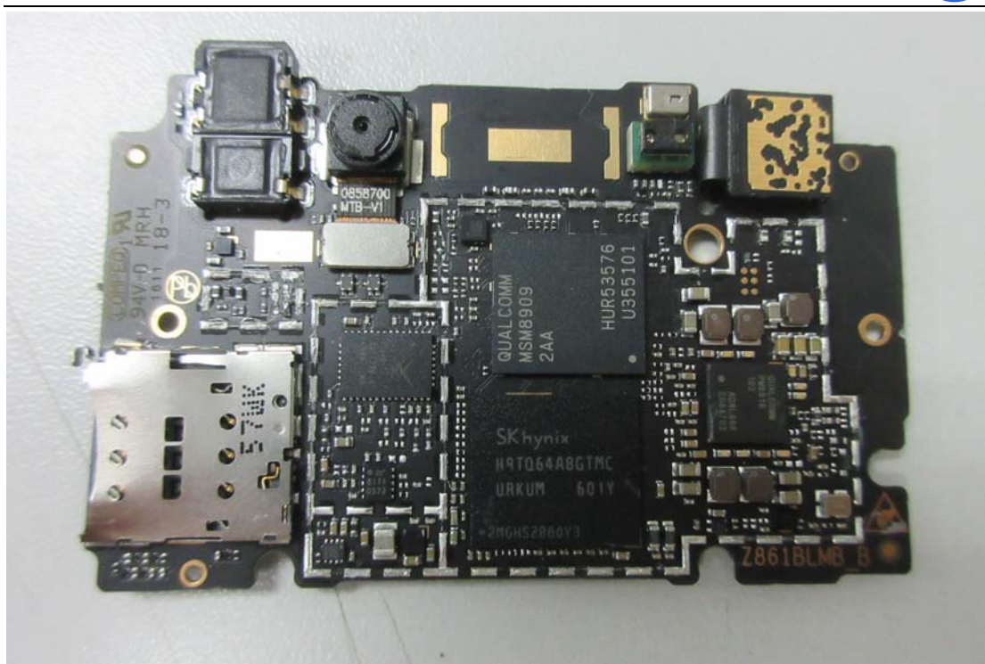
4. added board front view
