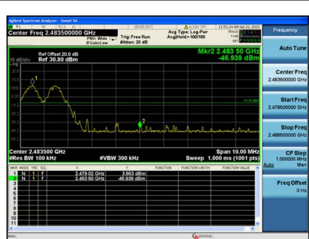
CH78(Hopping on)
