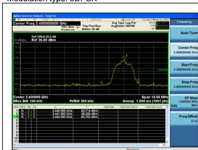
CH0(Hopping off)
