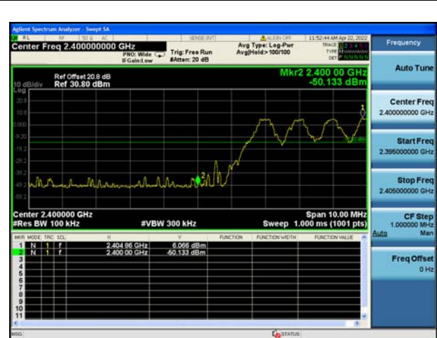
CH0(Hopping on)
