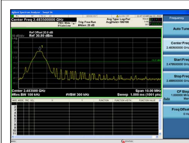
CH78(Hopping off)
