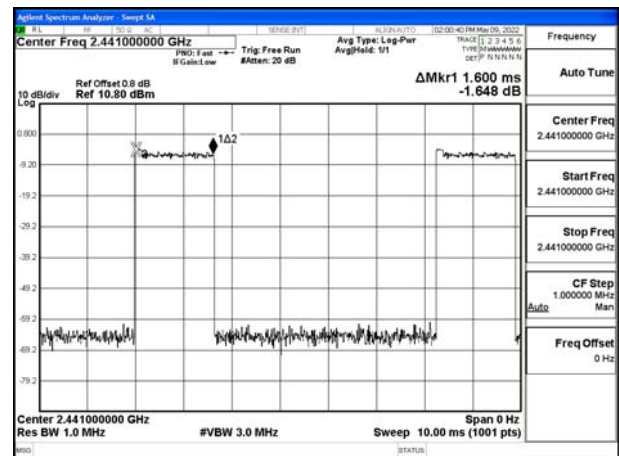
Modulation: 8DPSK 3DH3 2441MHz
