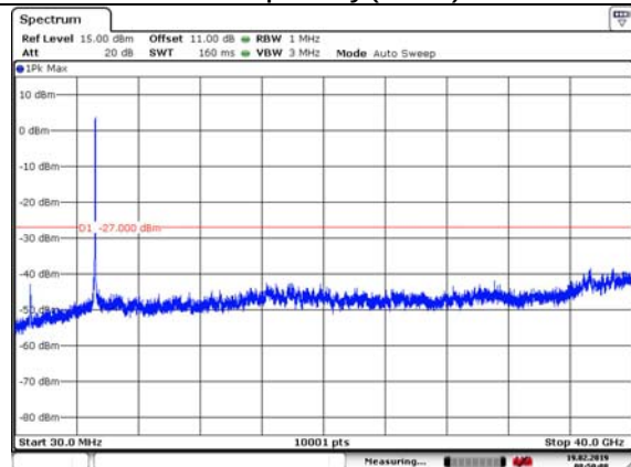
802.11ac HT80 (MIMO Ant2) Carrier frequency(MHz):5210
