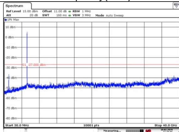
802.11n HT40 (MIMO Ant2) Carrier frequency(MHz):5230
