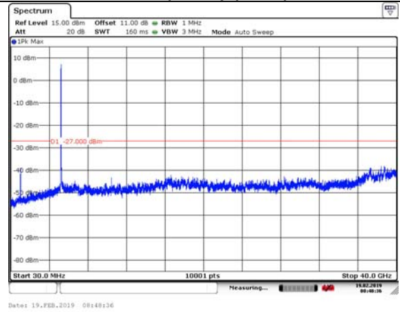
802.11n HT40 (SISO Ant2) Carrier frequency(MHz):5230
