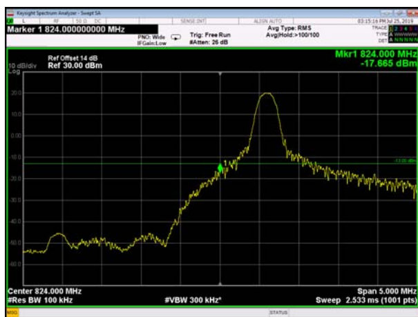
LowRange_FDD05_10MHz_829_fullRB _Low_QPSK
