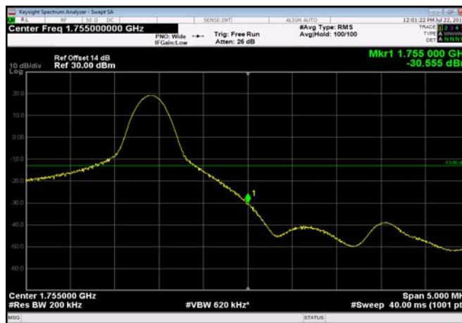
HighRange_FDD04_20MHz_1745_OneRB _high_QPSK
