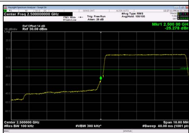
LowRange_FDD07_5MHz_2502.5_fullRB _Low_QPSK
