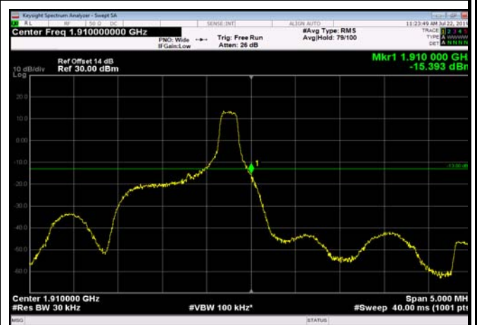
HighRange_FDD02_1.4MHz_1909.3 _fullRB_High_Q16
