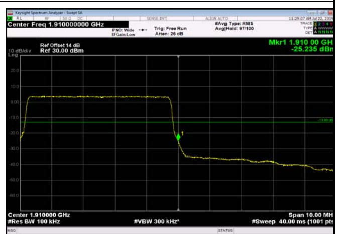
HighRange_FDD02_10MHz_1905_OneRB _high_Q16
