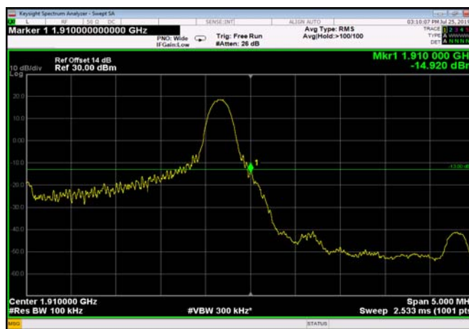
HighRange_FDD02_5MHz_1907.5_OneRB _high_QPSK
