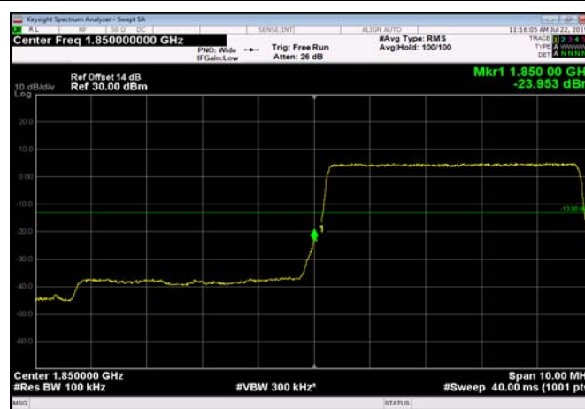
LowRange_FDD02_10MHz_1855_OneRB _low_QPSK
