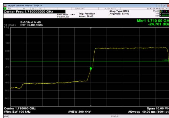
LowRange_FDD04_10MHz_1715_OneRB _low_QPSK
