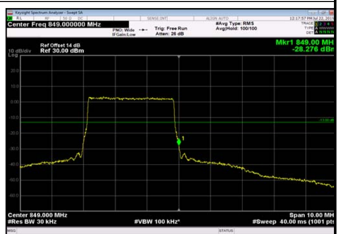
HighRange_FDD05_5MHz_846.5_OneRB _high_Q16
