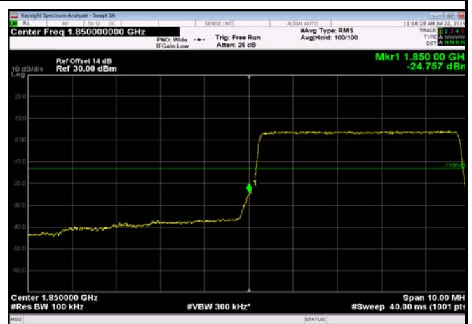
LowRange_FDD02_10MHz_1855_OneRB _low_Q16
