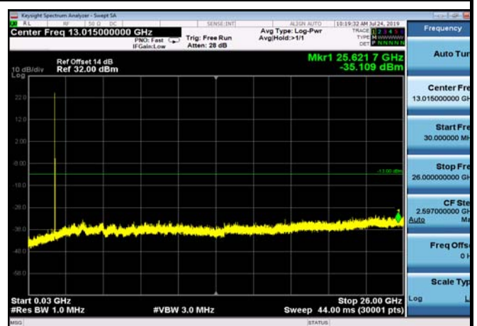
FDD02_MidRange_5MHz_30MHz~26GHz
