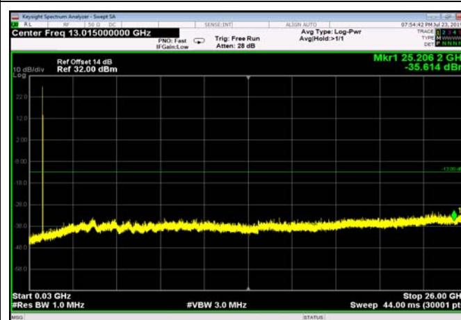
FDD05_HighRange_10MHz_30MHz~26GHz
