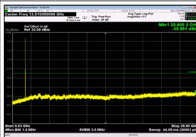
FDD02_LowRange_15MHz_30MHz~26GHz
