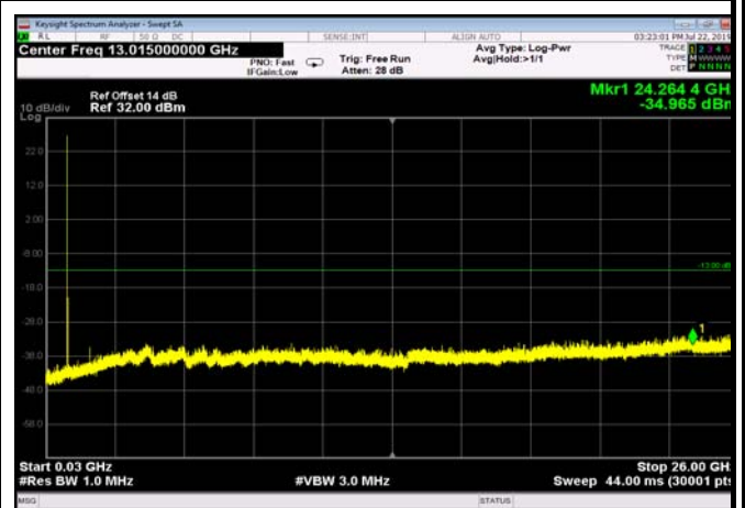
FDD07_HighRange_10MHz_30MHz~26GHz
