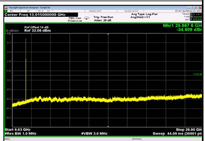
FDD02_MidRange_20MHz_30MHz~26GHz
