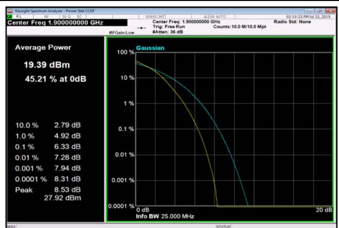
FDD02_HighRange_20MHz_1900_fullRB _Q16
