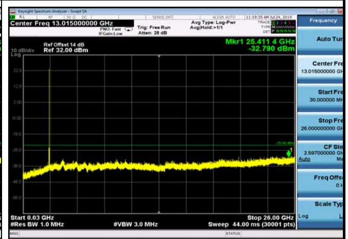
FDD07_MidRange_20MHz_30MHz~26GHz
