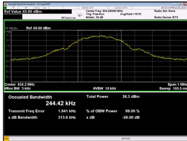
(Plot A1: GPRS 850MHz Channel = 128 Occupied bandwidth)
