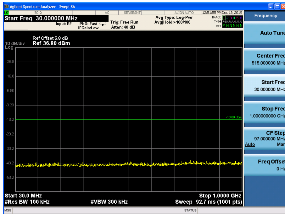
Channel 661, 30MHz~1GHz
