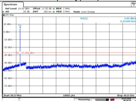
802.11ac VHT80 (MIMO Ant1) Carrier frequency(MHz):5210
