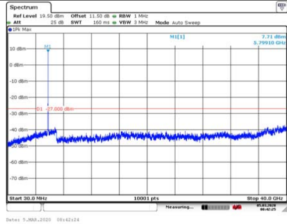
802.11ac VHT80 (MIMO Ant0) Carrier frequency(MHz):5775
