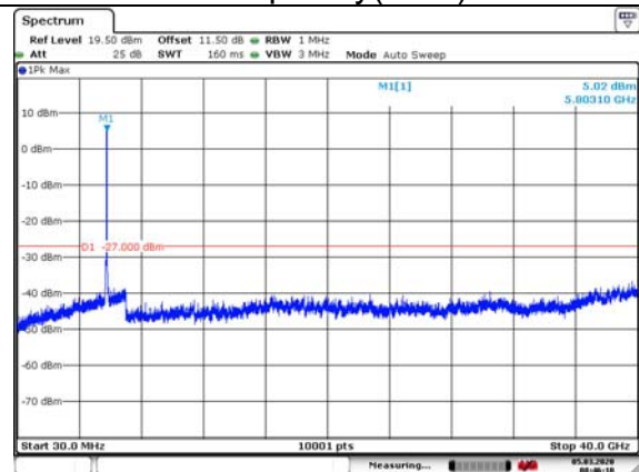
802.11ac VHT80 (MIMO Ant1) Carrier frequency(MHz):5775
