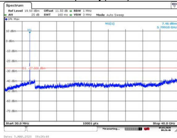
802.11ac VHT80 (SISO Ant0) Carrier frequency(MHz):5775
