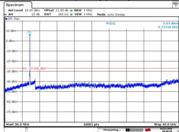
802.11ac VHT80 (MIMO Ant0) Carrier frequency(MHz):5775
