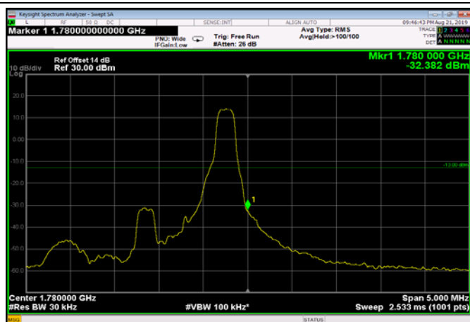
HighRange_FDD66_1.4MHz_1779.3 _fullRB_High_Q16
