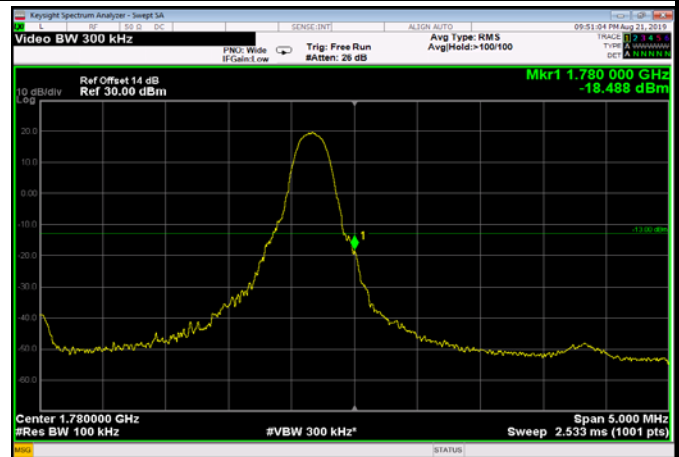
HighRange_FDD66_5MHz_1777.5_fullRB _High_Q16
