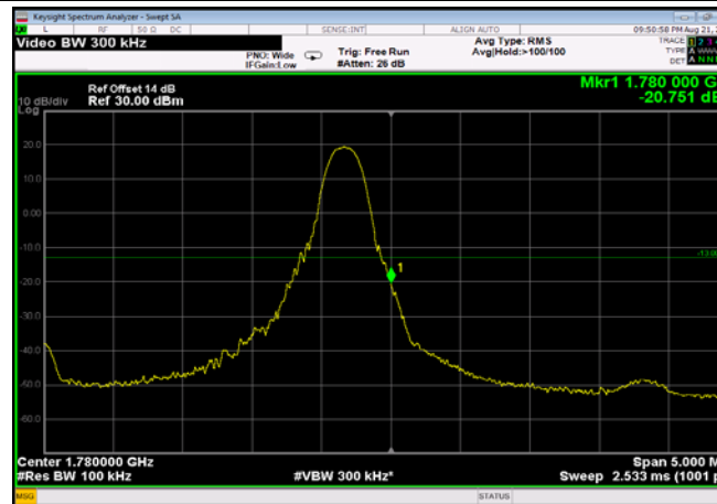
HighRange_FDD66_5MHz_1777.5_fullRB _High_QPSK
