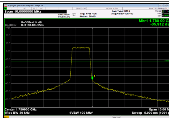
HighRange_FDD66_1.4MHz_1779.3 _fullRB_High_QPSK
