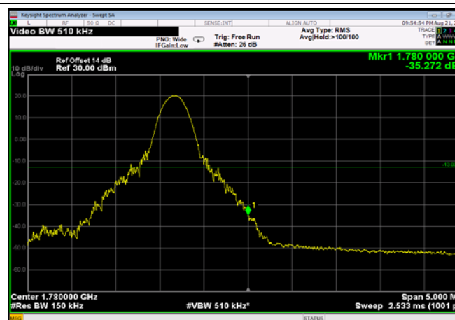
HighRange_FDD66_15MHz_1772.5_OneRB _High_QPSK
