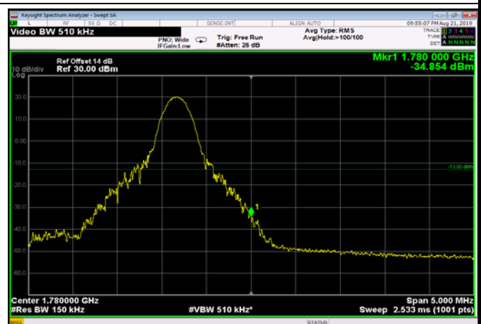
HighRange_FDD66_15MHz_1772.5_OneRB _High_Q16
