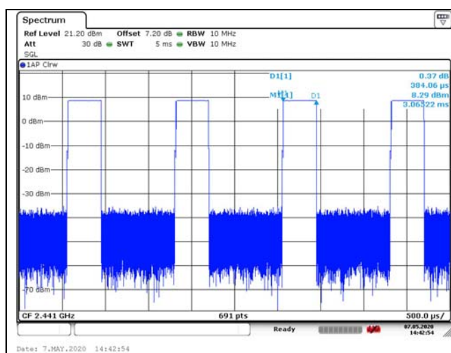
Modulation type: GFSK DH1 2441MHz
