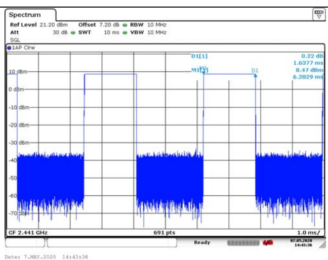
Modulation type: GFSK DH3 2441MHz
