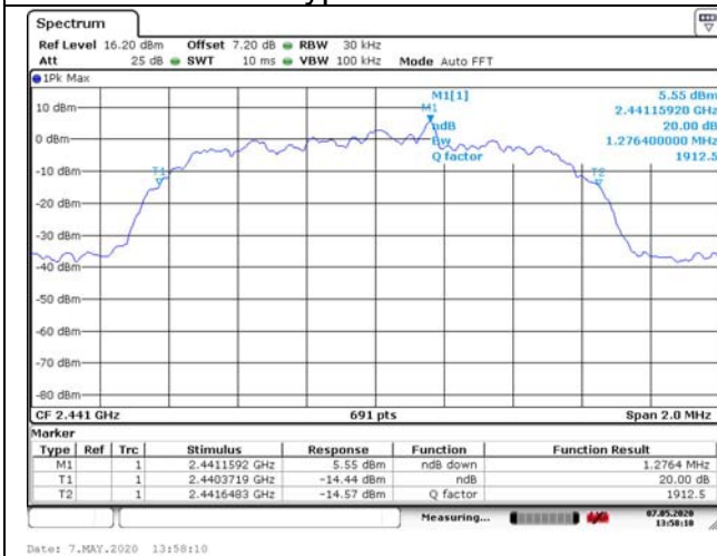
Modulation type: \pi/4 DQPSK 2441MHz
