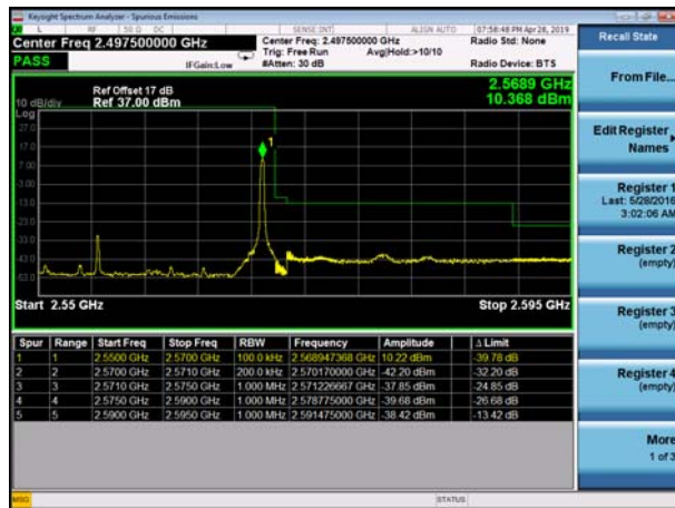
LowRange_FDD07_10+20MHz_FullRB QPSK
