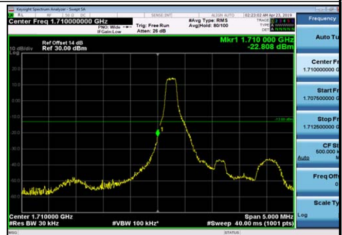
LowRange_FDD66_1.4MHz_1710.7_OneRB _low_Q16
