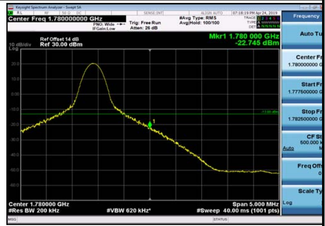
HighRange_FDD66_20MHz_1770_OneRB _high_Q16
