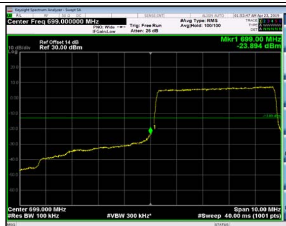
LowRange_FDD12_5MHz_701.5_fullRB _Low_QPSK
