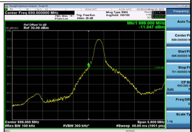
LowRange_FDD12_5MHz_701.5_fullRB _Low_Q16
