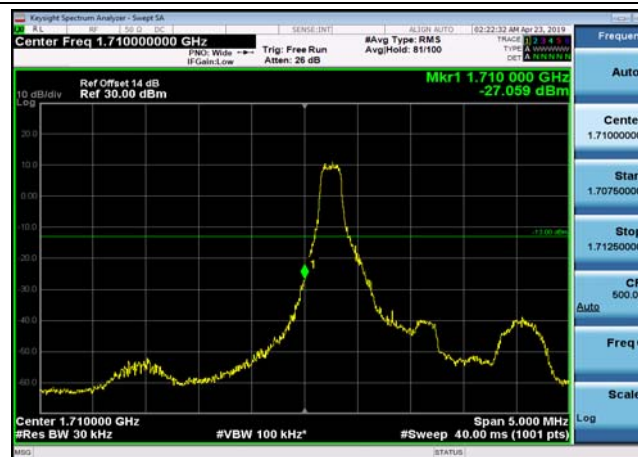
LowRange_FDD66_1.4MHz_1710.7_OneRB _low_QPSK
