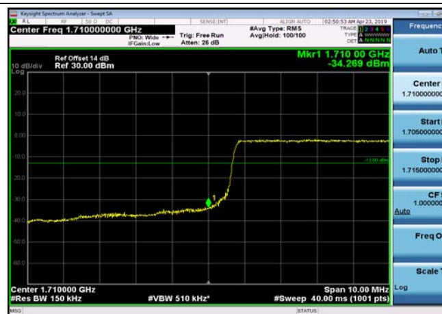
LowRange_FDD66_15MHz_1717.5_fullRB _Low_QPSK
