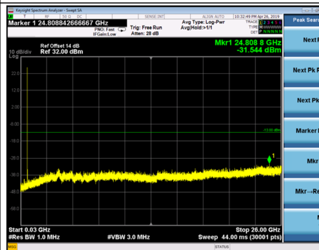
FDD12_HighRange_1.4MHz_30MHz~26GHz
