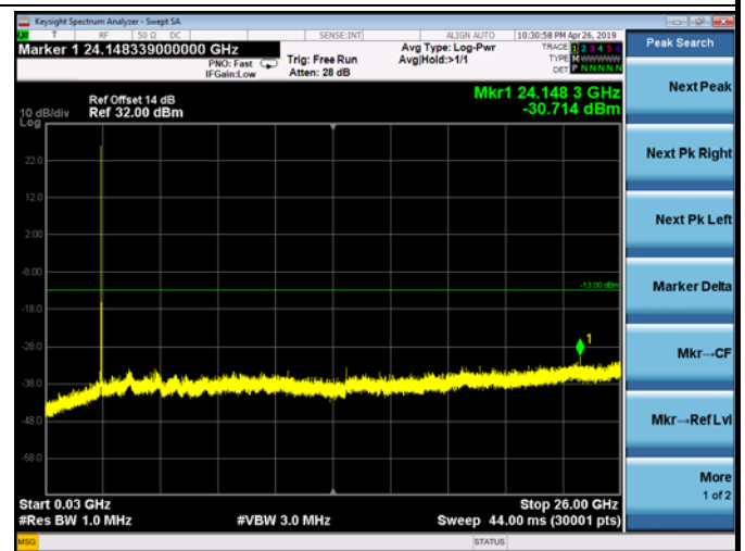
FDD12_MidRange_1.4MHz_30MHz~26GHz
