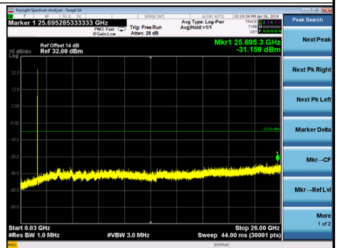
FDD04_LowRange_20MHz_30MHz~26GHz
