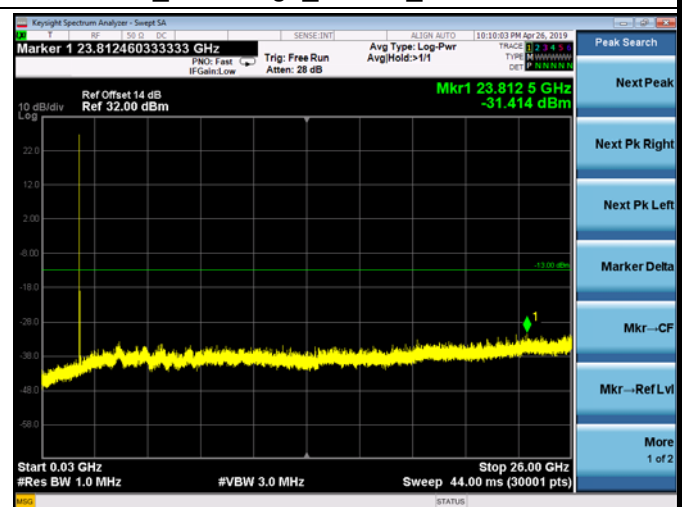
FDD02_LowRange_10MHz_30MHz~26GHz
