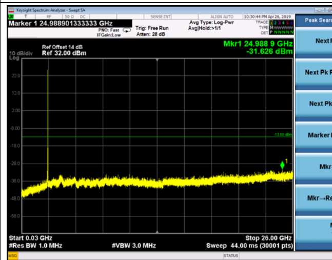
FDD12_LowRange_1.4MHz_30MHz~26GHz
