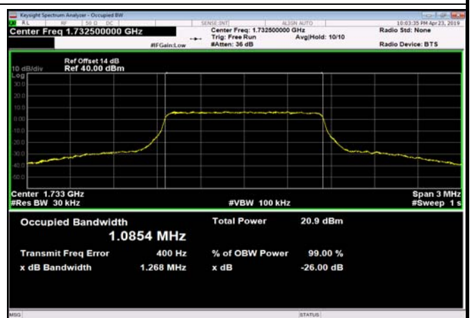
FDD04_MidRange_1.4MHz_1732.5MHz_Q16
