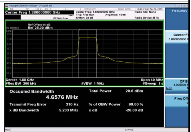
FDD02_MidRange_20_1880_Q16
