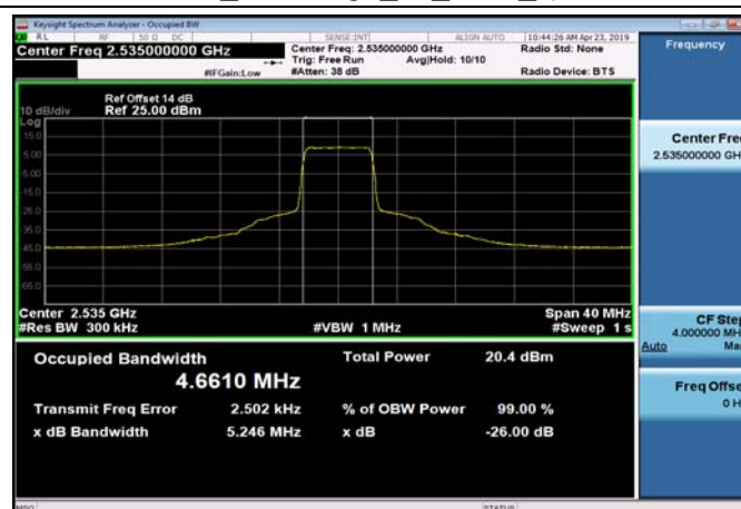
FDD07_MidRange_15_2535_QPSK
