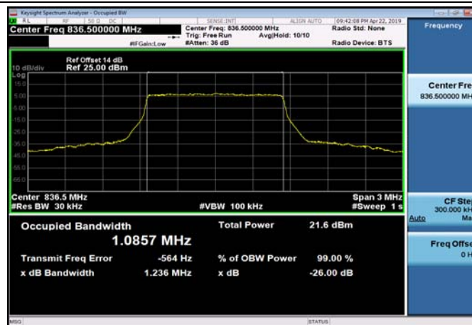
FDD05_MidRange_1.4MHz_836.5MHz _Q16
