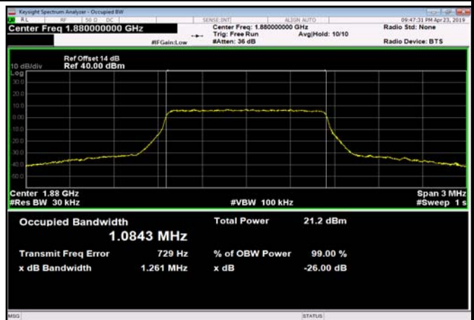
FDD02_MidRange_3MHz_1880MHz_Q16
