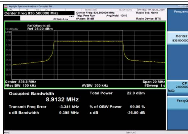
FDD05_MidRange_10MHz_836.5MHz_QPSK
