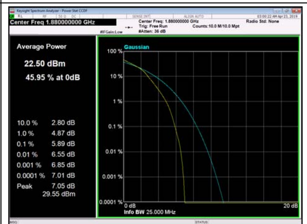
FDD02_HighRange_20MHz_1900_fullRB _Q16
