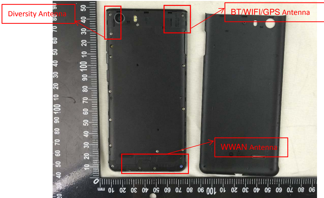
EUT UNCOVER VIEW 1
