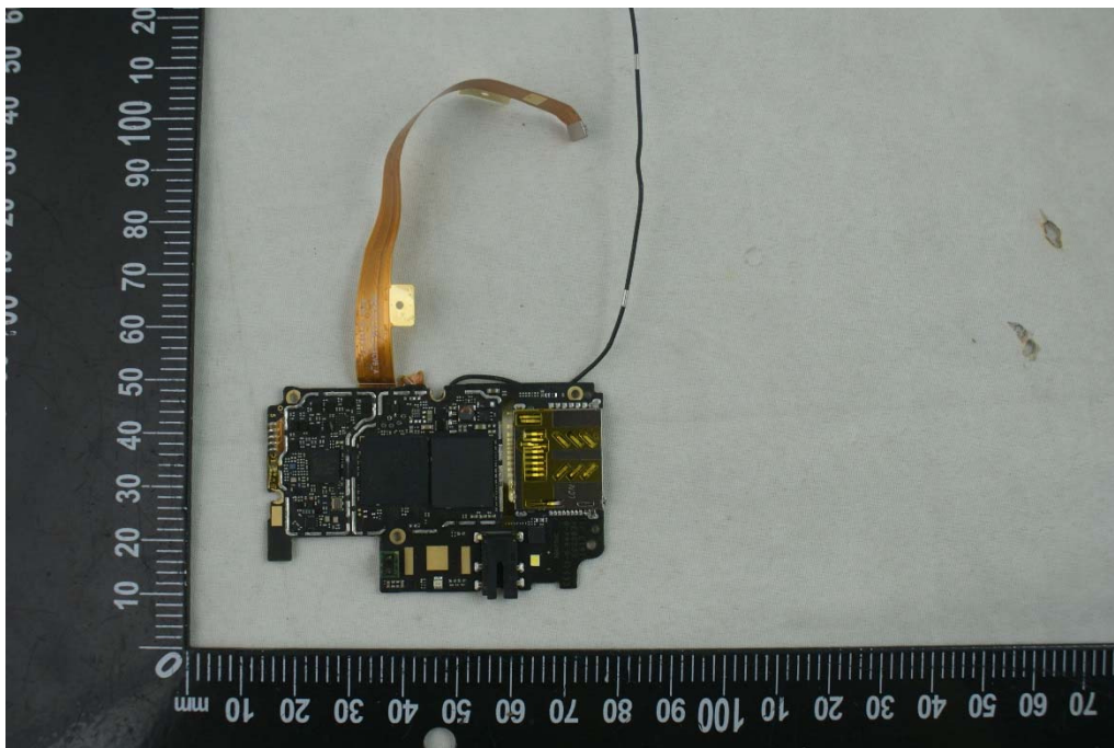
MAIN BOARD 2 TOP VIEW
