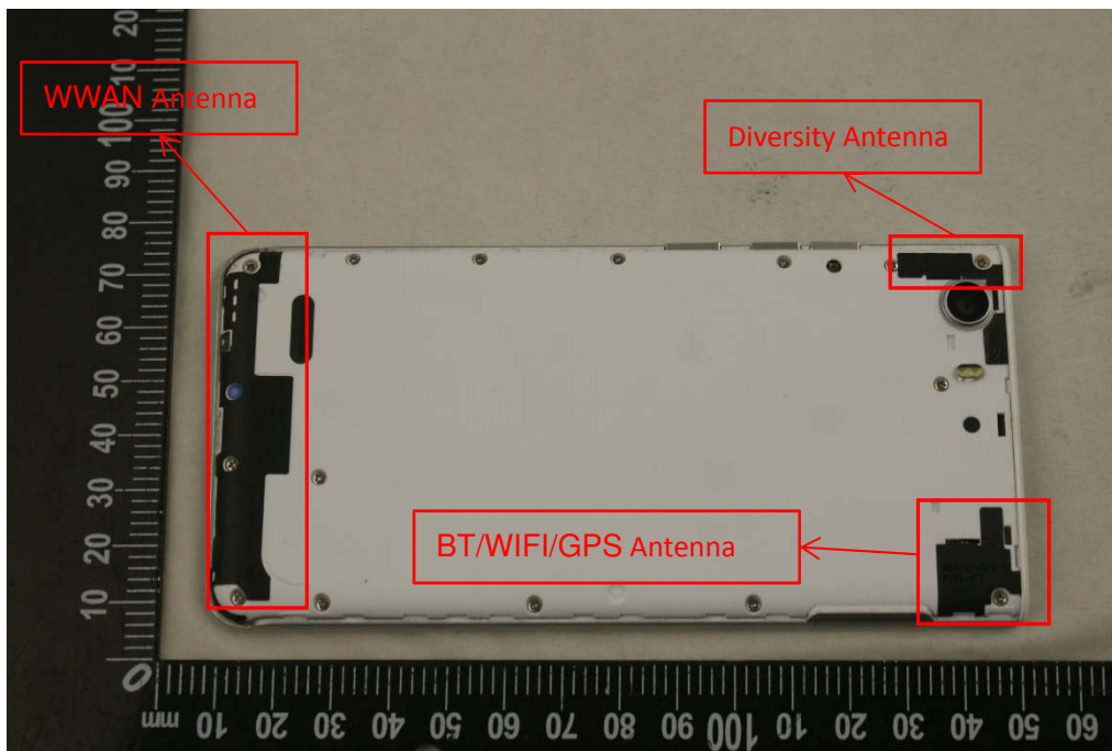
EUT UNCOVER VIEW 2
