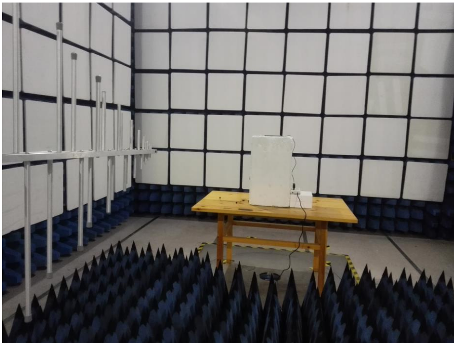
Below 1 GHz
