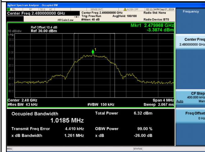
99% Occupied Bandwidth - High CH 2480
