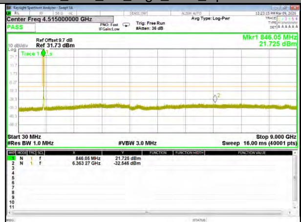
B5_Q16_5M_High_CDT_Spurious
