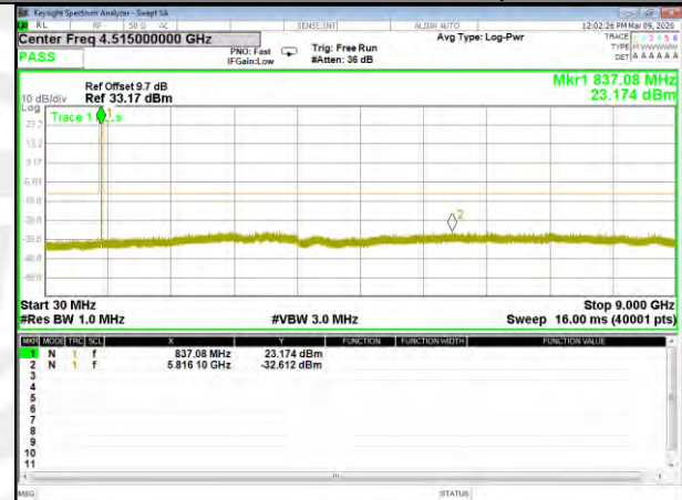
B5_Q16_1.4M_High_CDT_Spurious
