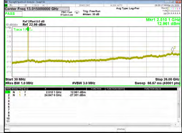
B7_Q16_15M_Mid_CDT_Spurious
