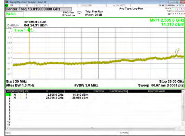
B7_QPSK_10M_Mid_CDT_Spurious
