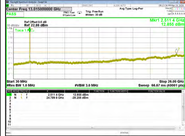
B7_QPSK_20M_Mid_CDT_Spurious
