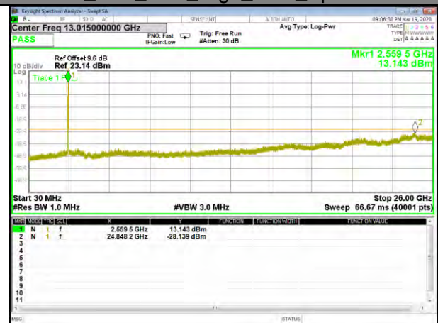
B7_Q16_15M_High_CDT_Spurious
