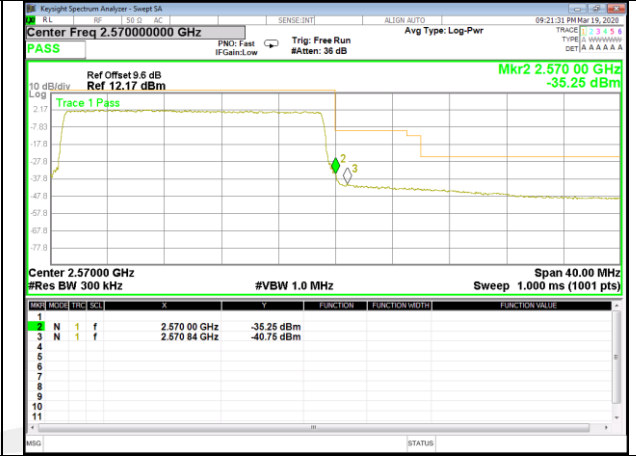
B7_Q16_20M_High_Full-RB_Bedge
