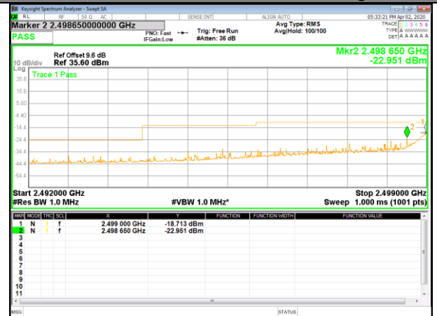
B7_Q16_5M_Low_Full-RB_Bedge
