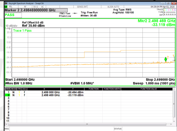
B7_QPSK_10M_High_Full-RB_Bedge
