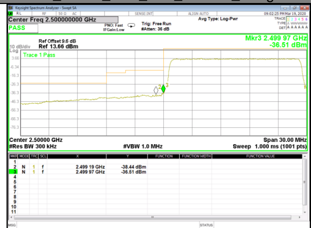
B7_QPSK_15M_Low_Full-RB_Bedge
