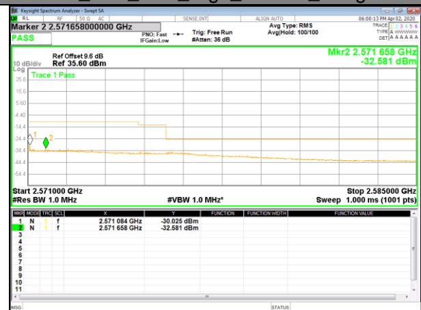
B7_Q16_15M_High_Full-RB_Bedge
