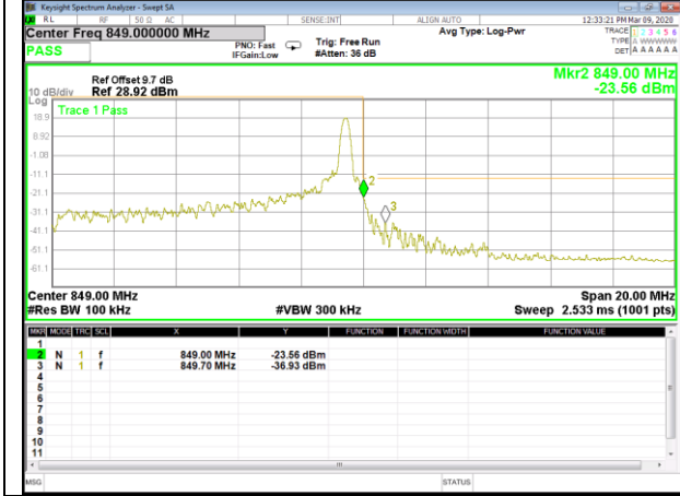
B5_Q16_10M_High_1-RB_Bedge
