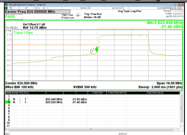
B5_QPSK_5M_Low_Full-RB_Bedge
