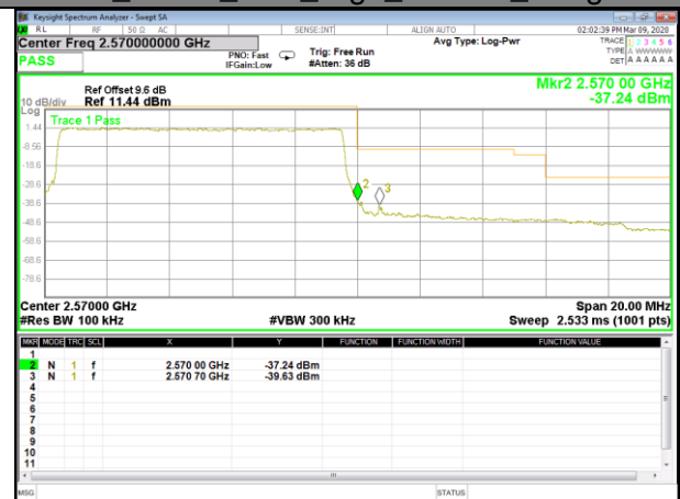
B7_QPSK_10M_High_Full-RB_Bedge
