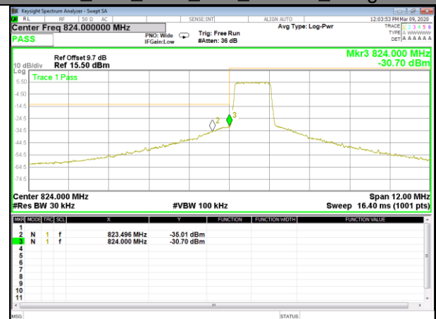
B5_Q16_1.4M_Low_Full-RB_Bedge
