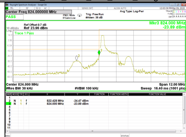
B5_Q16_1.4M_Low_1-RB_Bedge
