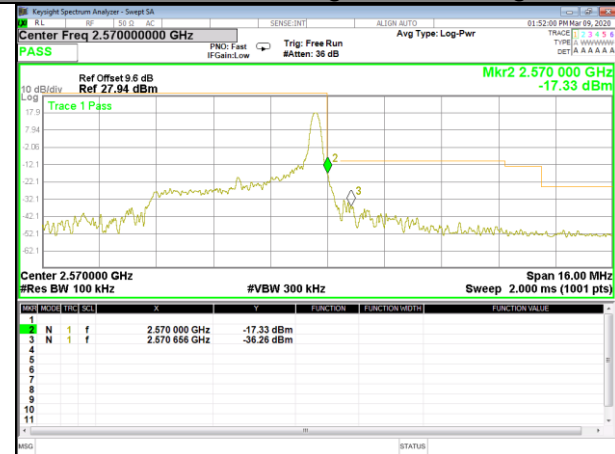
B7_Q16_5M_Low_1-RB_Bedge
