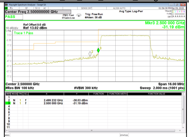
B7_Q16_5M_Low_Full-RB_Bedge
