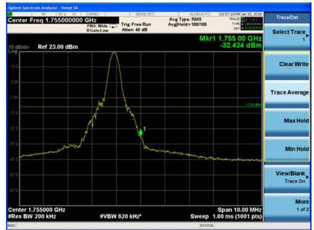
LTE Band 4 QPSK 20MHz CH-High, 100%RB
