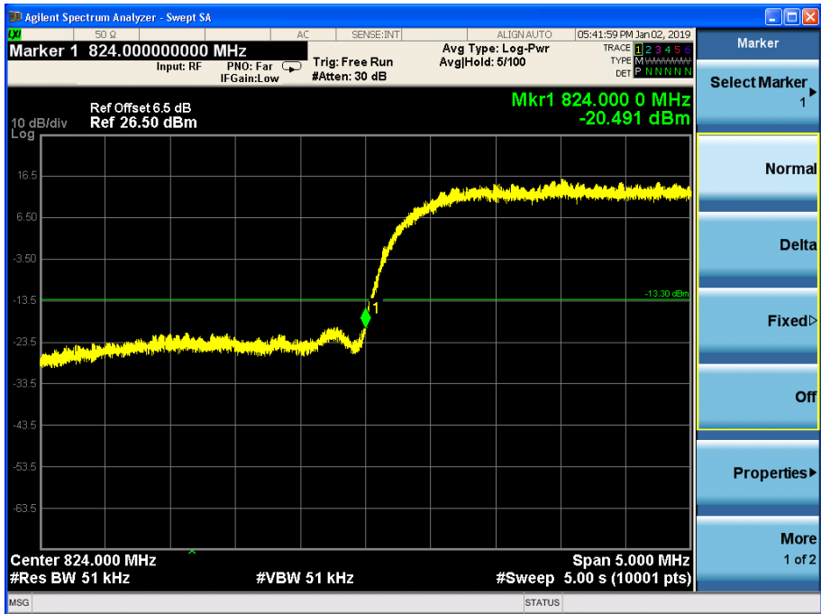
Channel 4132
