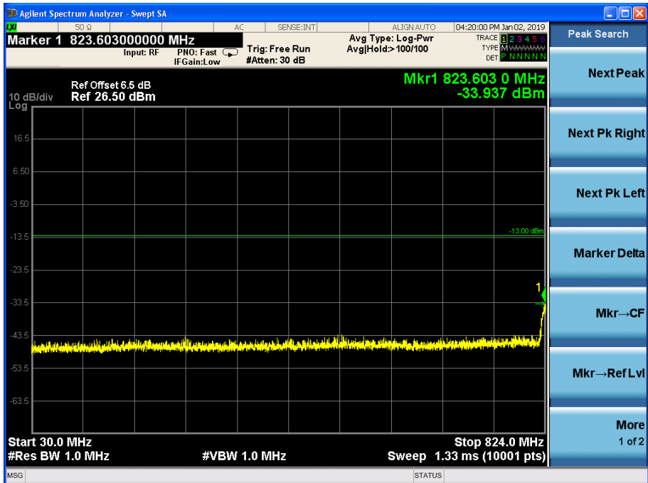
Channel 4183, 30MHz~824MHz
