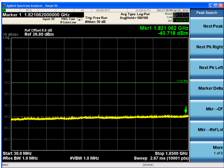
Channel 9400, 30MHz~1850MHz
