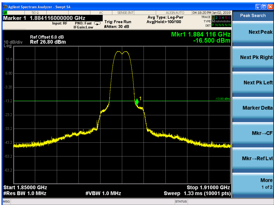
Channel 9400, 1850MHz~1910MHz
