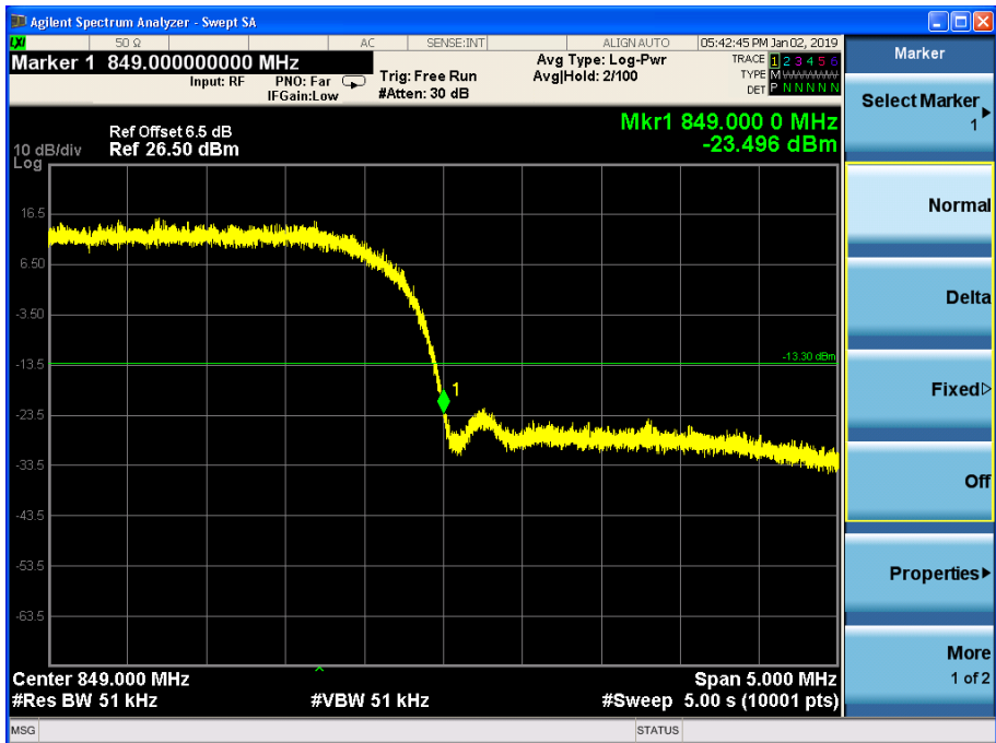
Channel 4233
