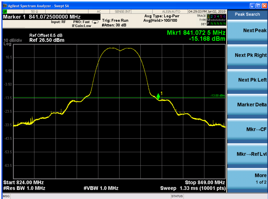
Channel 4183, 824MHz~849MHz
