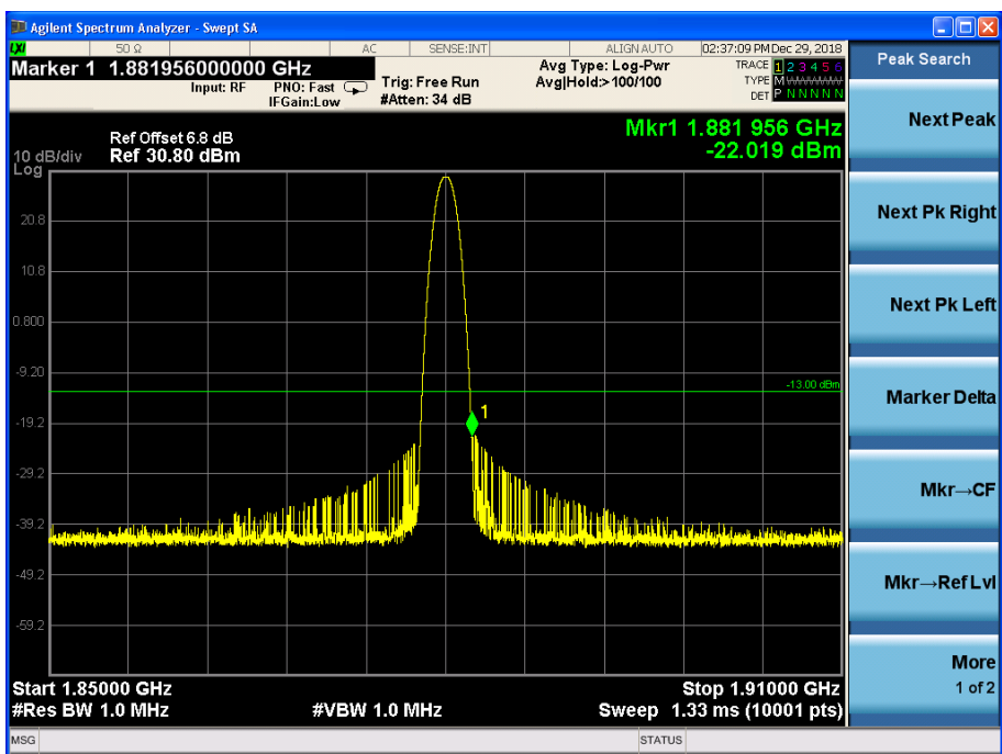
Channel 661, 1850MHz~1910MHz
