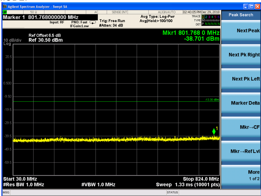
Channel 189, 30MHz~824MHz
