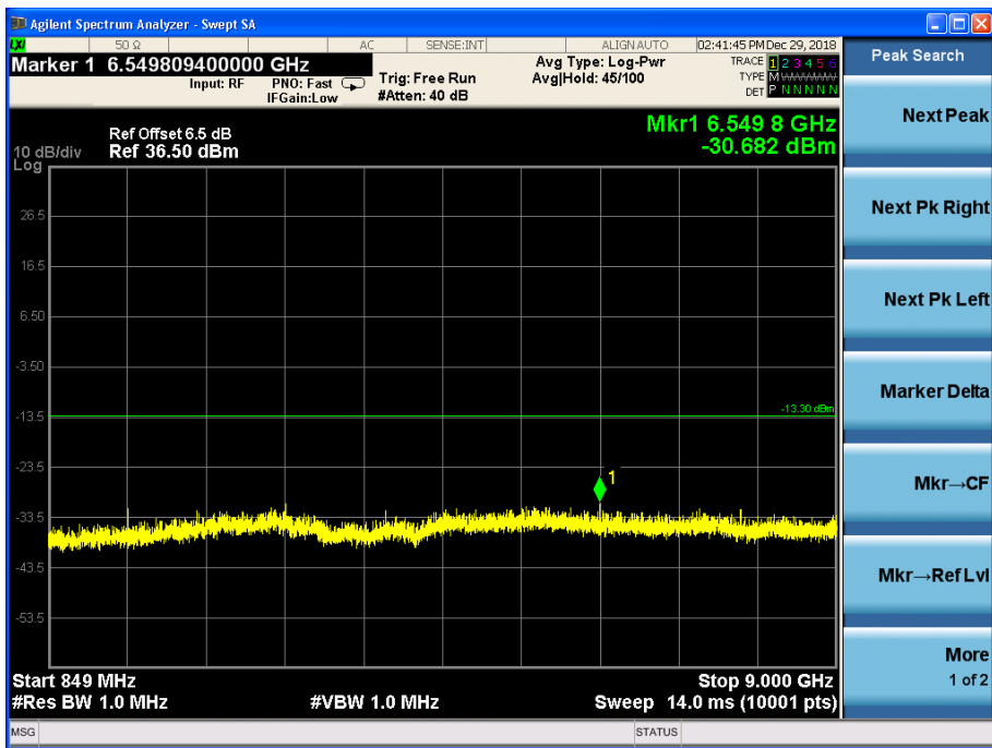
Channel 189, 849MHz~9GHz
