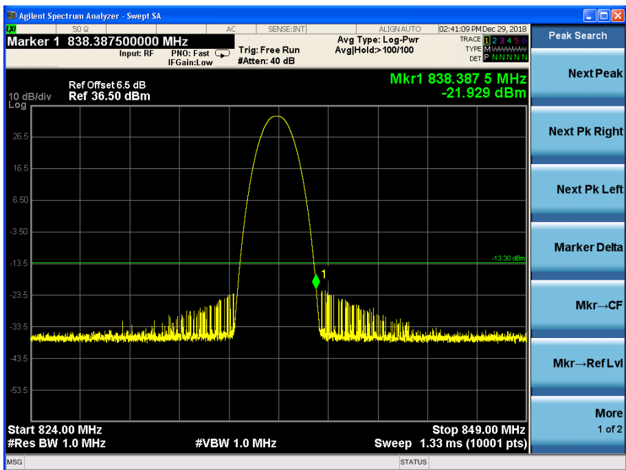
Channel 189, 824MHz~849MHz
