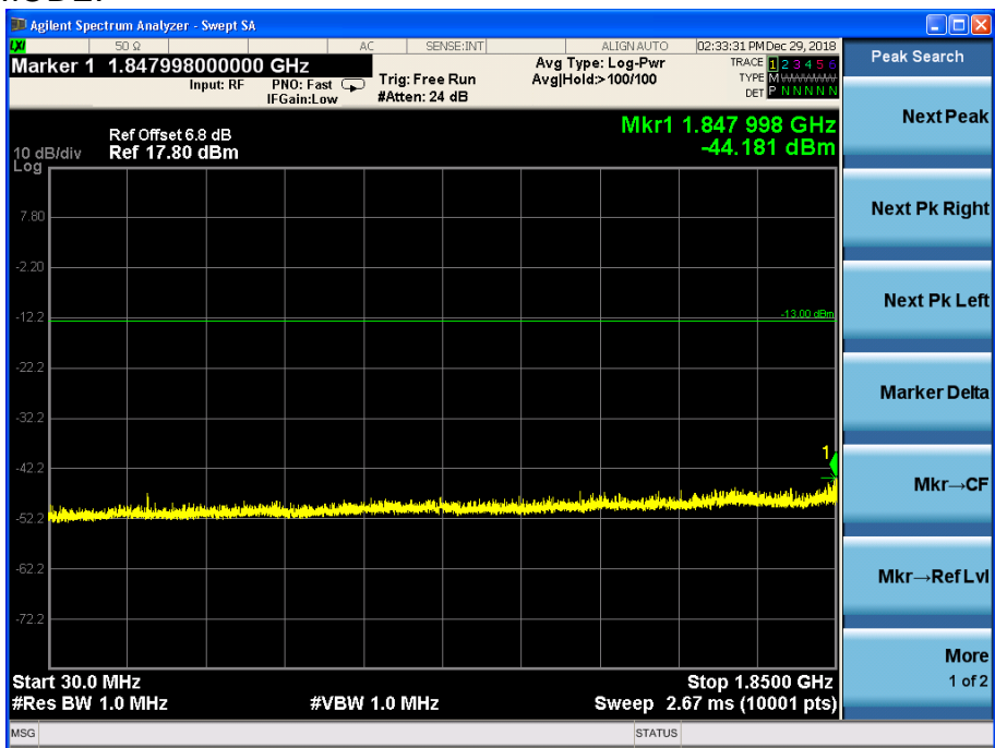
Channel 661, 30MHz~1850MHz
