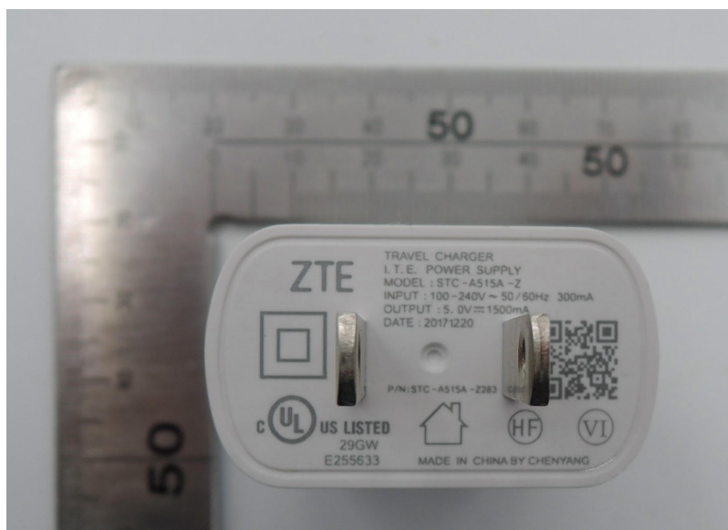
CHARGER View (Jiangsu Chenyang Electro Co.,Ltd)
