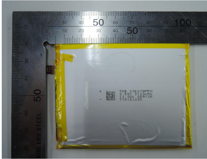
The battery view (Zhongshan Tianmao Battery Co.,LTD)
