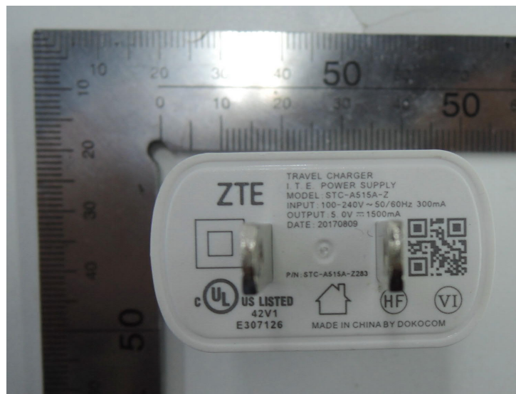
CHARGER View (Shenzhen Dokocom Energy Technology Co.,Ltd)
