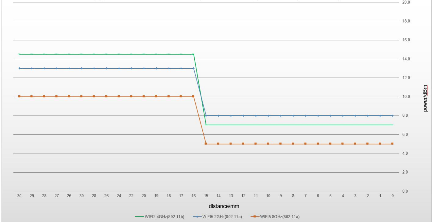
Trigger distance evaluation(Back moving towards phantom )
