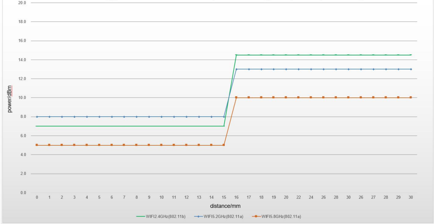
Trigger distance evaluation(Back moving away from phantom )
