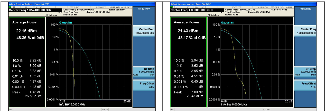
Channel 9262
