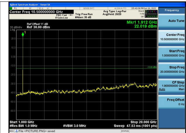
Channel 9262 1GHz~20GHz(dBm)
