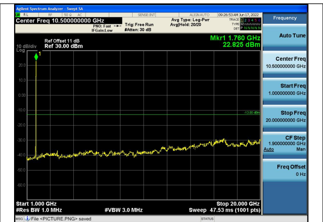
Channel 1312 1GHz~20GHz(dBm)
