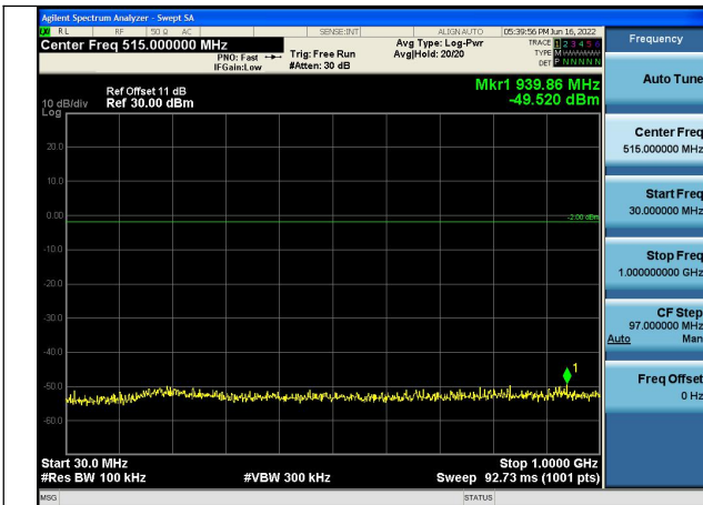
Channel 9262 30MHz~1GHz(dBm)
