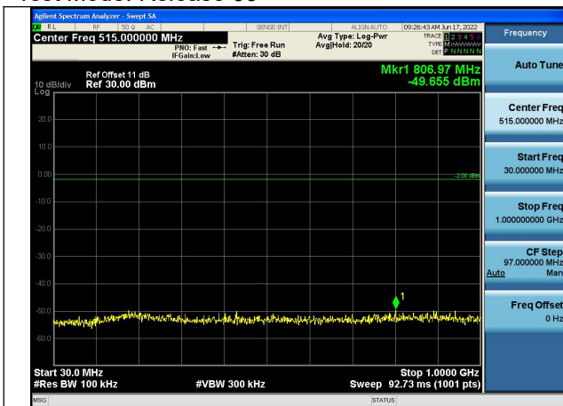
Channel 1312 30MHz~1GHz(dBm)
