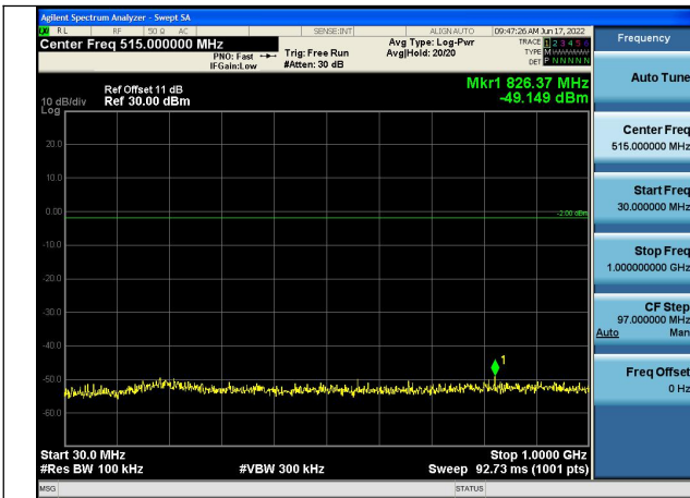
Channel 1312 30MHz~1GHz(dBm)
