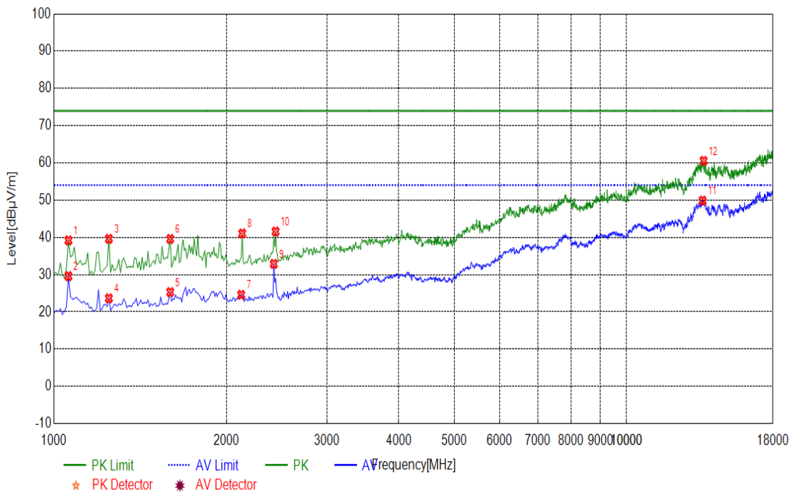
(Plot F: Test Antenna Vertical 1G – 18G)
