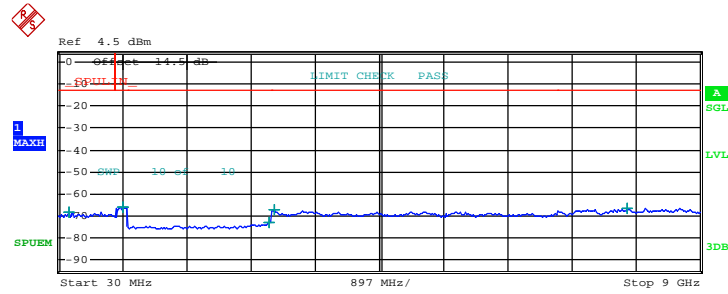
Conducted Emission Plot between on Channel 476 (817.9MHz)
