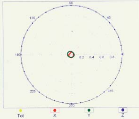
f=2500 MHz,R22,90°
