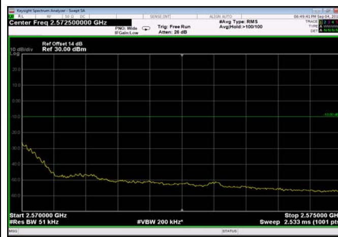
FDD07_15MHz_2562.5_Q16_OneRB_high _ExtraBands_Range_2570~2575
