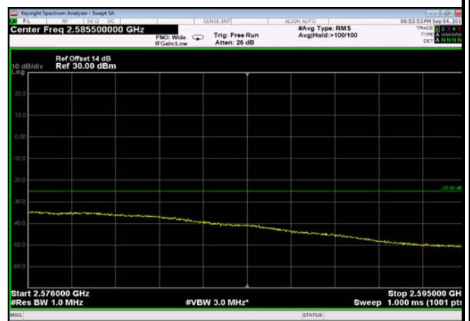
HighRange_FDD07_20MHz_2560_OneRB _high_Q16
