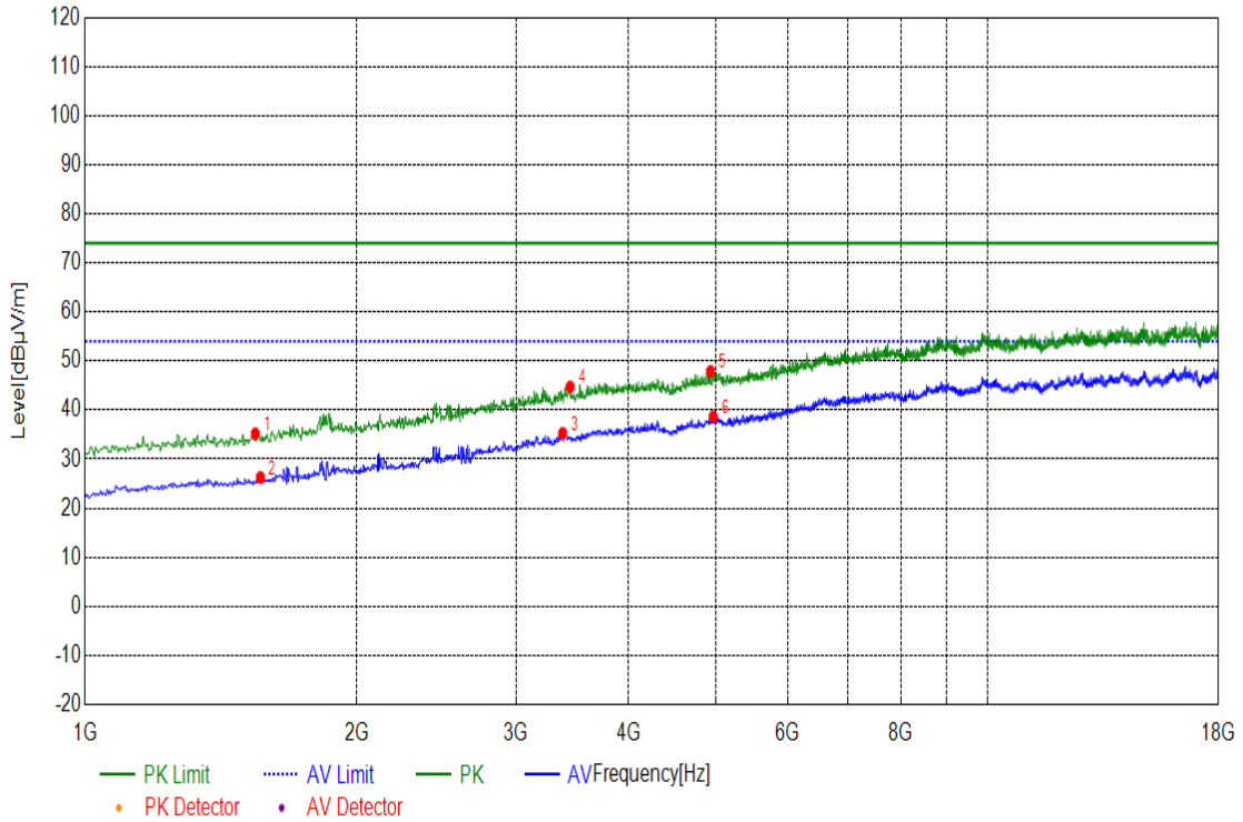
(Plot M: Test Antenna Horizontal 1G – 18G)
