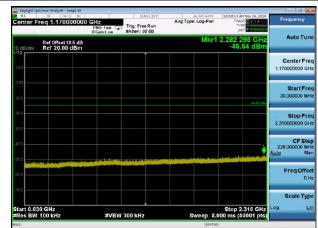
,Plot 3,30MHz~2310MHz-802.11g,2462MHz
