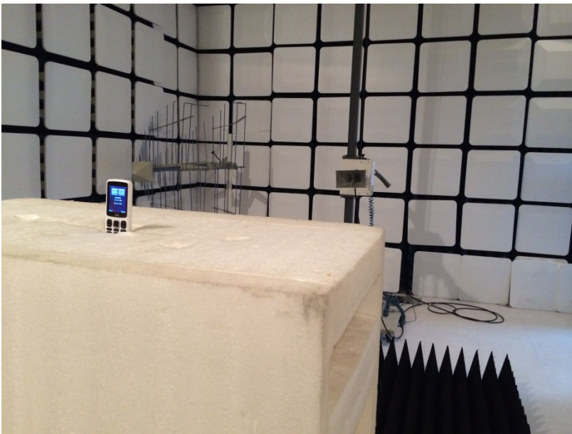
Radiated Emission
