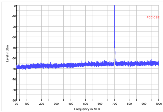
LTE Band 12 1.4MHz CH-Low 30MHz~1GHz
