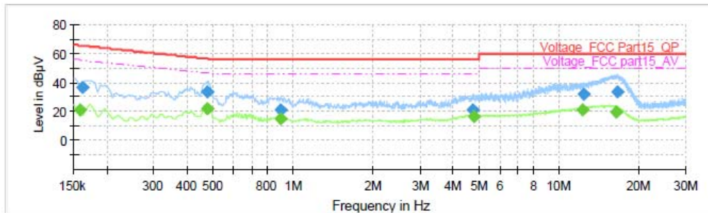
L_0.15-30MHz
