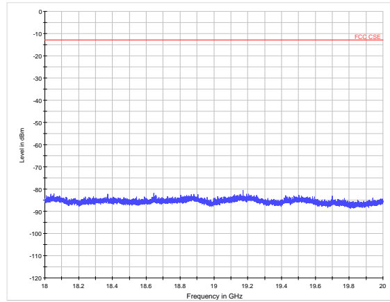
WCDMA Band II CH-Middle 18GHz~20GHz
