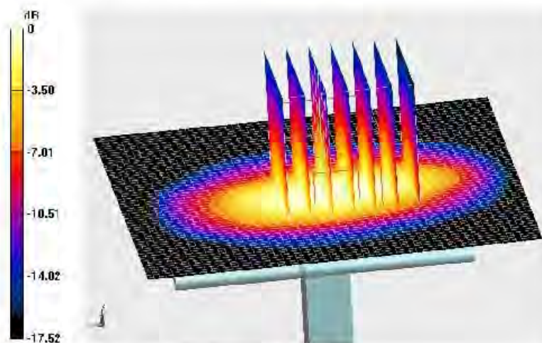
0 dB = 12.2 W/kg = 10.86 dBW/kg
