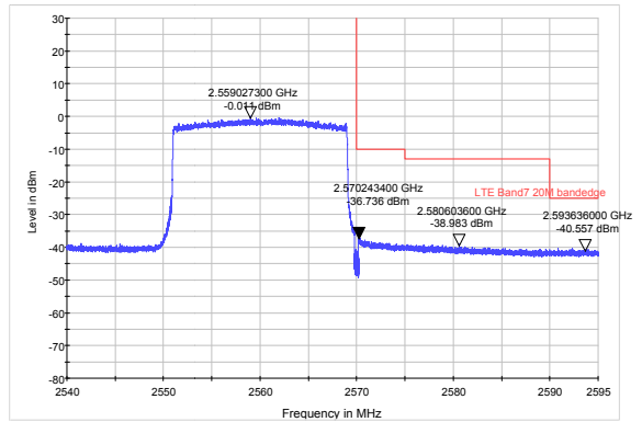
LTE Band 7 16QAM 20MHz CH-High, 100%RB
