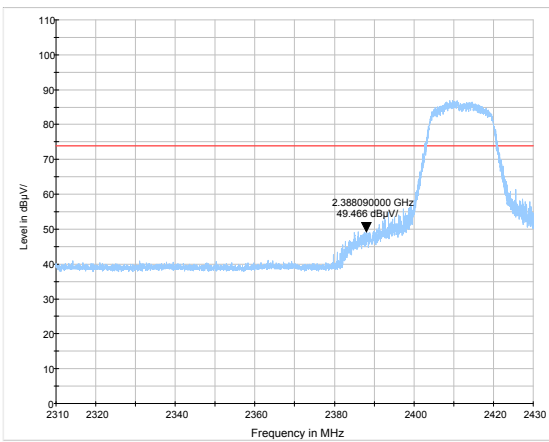
802.11g-Channel 1: Peak
